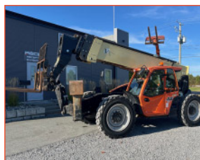
JLG G10-55A 2016
